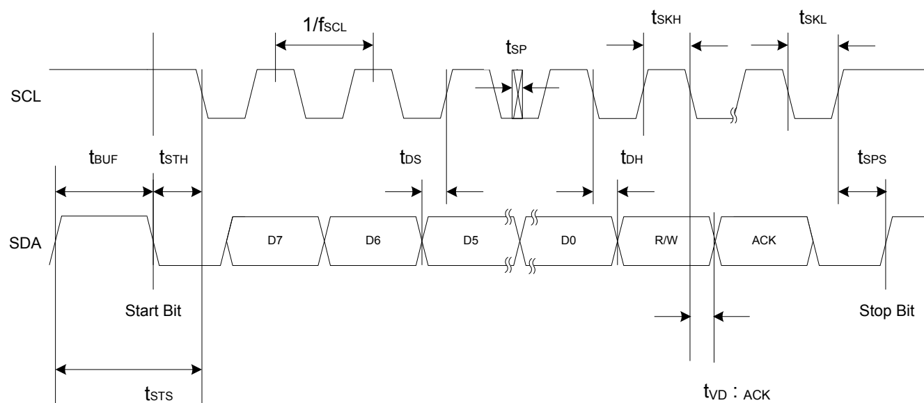
Figure 1. I²C Interface Timing Diagram
