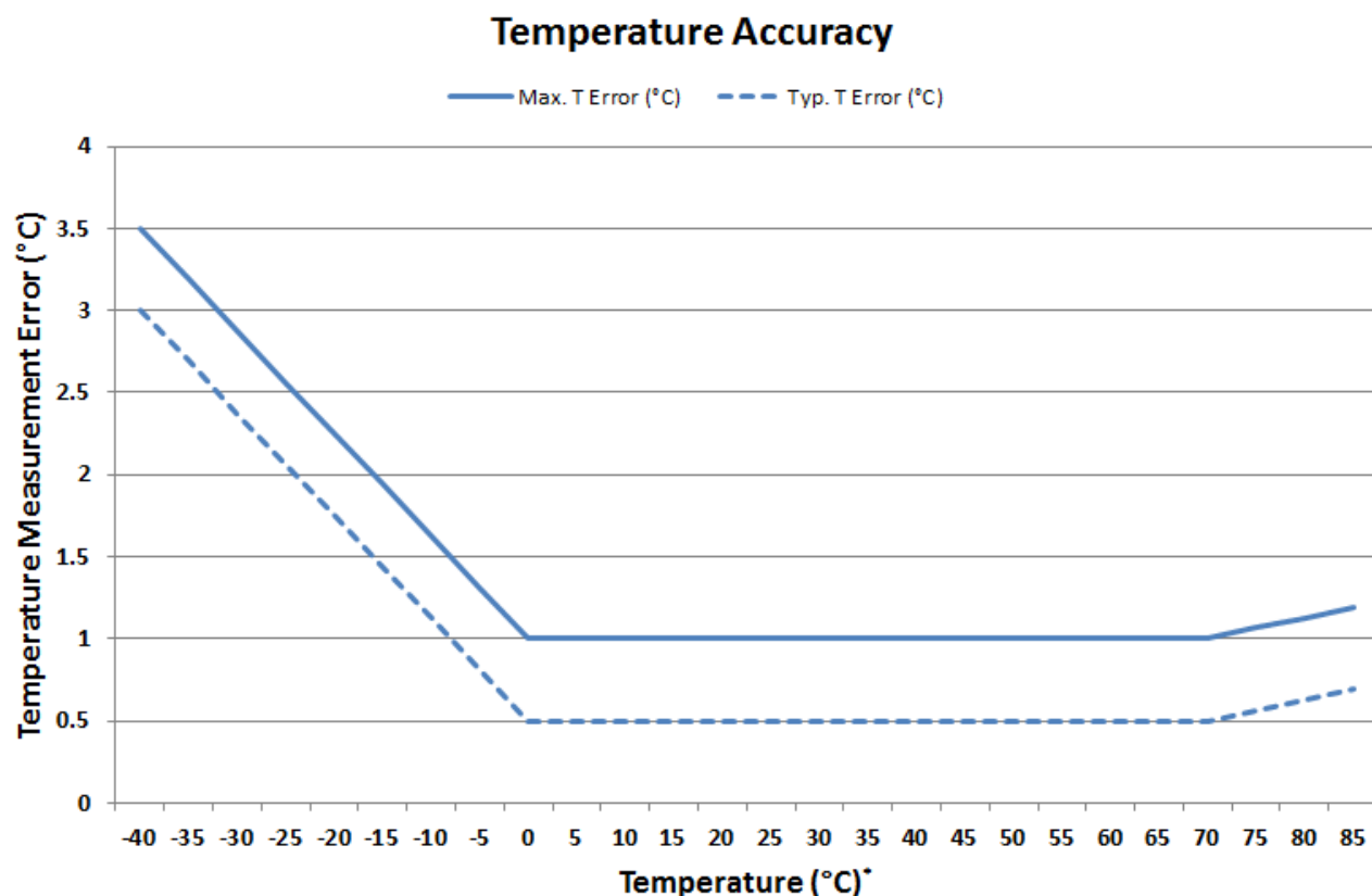
Figure 3. Temperature Accuracy*
